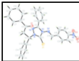
Fig. 1. A view of a molecule of the title compound showing the atom-labelling scheme. Displacement ellipsoids are drawn at the 60% probability level.
